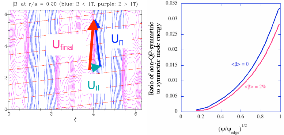
Fig.1 . Quasi-poloidal symmetry characteristics for QPS.
