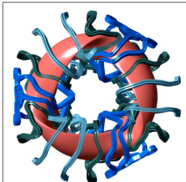
Fig. 1. NCSX Plasma and modular coils.
