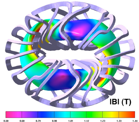
Fig. 2. Top view of QPS plasma and coils with |B| contours
